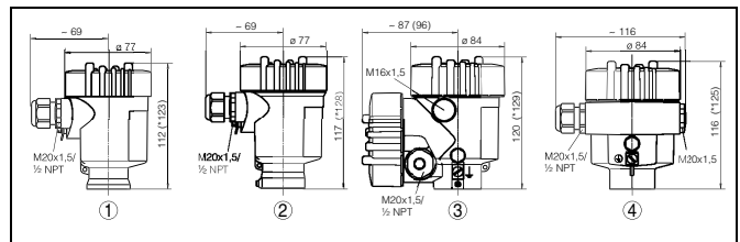
Fig. 50: Housing versions
