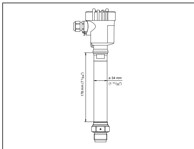
Fig. 55: Temperature adapter
