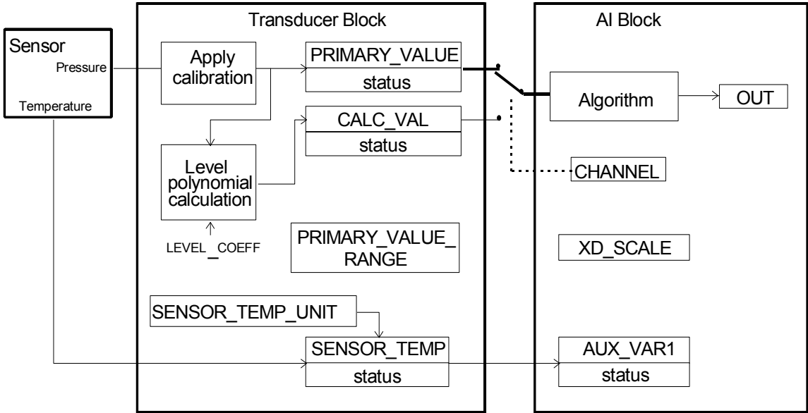
Figure 4 — Transducer and Analog Input Function Block Diagram
