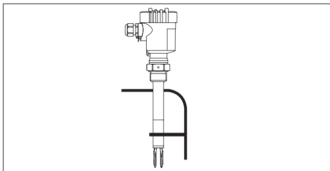
Fig. 10: Lateral support of VEGASWING 63
