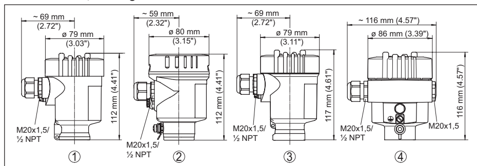
Fig. 37: Housing versions
