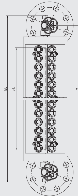
Version with valve head, top/bottom, model LGV-53
