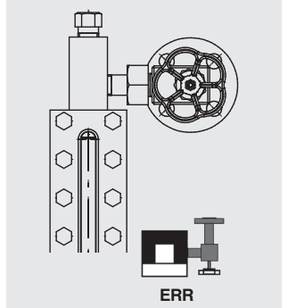
Angled valve Right mount (lateral)
