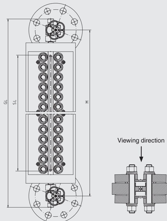
Version with valve head, top/bottom, model LGV-53
