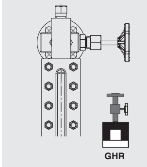
Angled valve Back mount, right-hand
