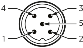
Figure 11 M12/5 Male Connector Pinout
