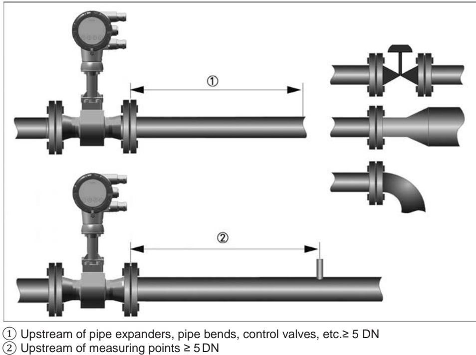
Figure 15: Minimum outlet sections
