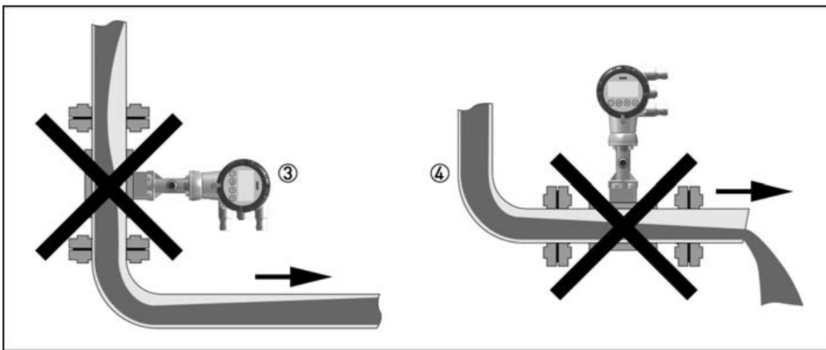
Figure 10: Downstream pipe and outlet
