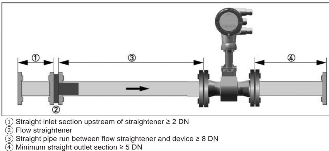
Figure 16: Flow straightener
