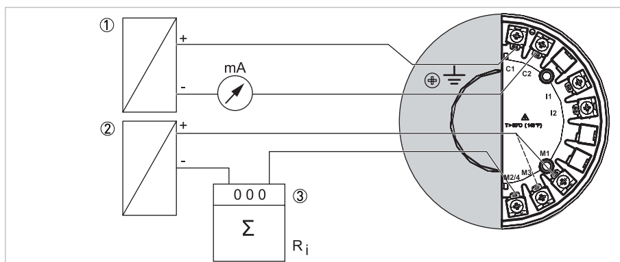
Figure 4-5: Electrical connection pulse output
