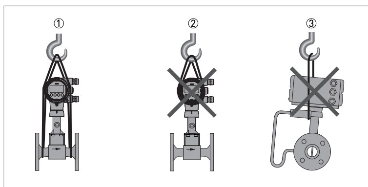
Figure 3-1: Transport instructions
