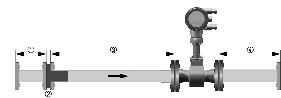
Figure 3-10: Flow straightener
