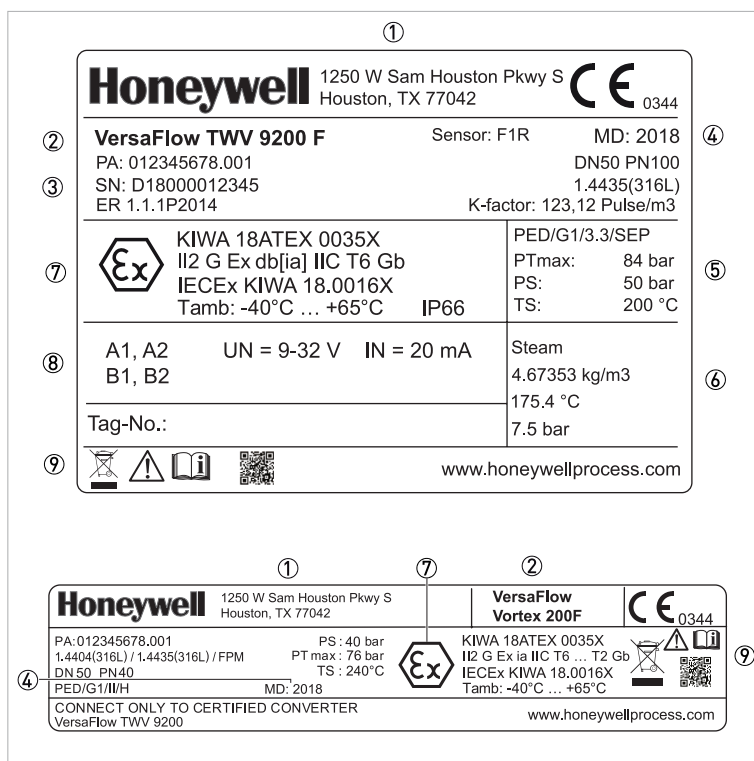
Figure 2-10: Example of a nameplate for the remote version
