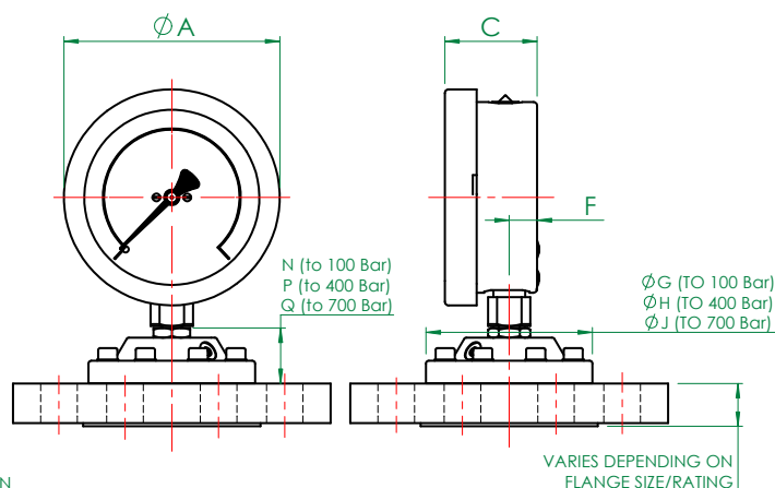
MODEL - 2033/F (above DN50/2") Flange Mounted - Rated as Flange to Maximum seal/chamber ratings
