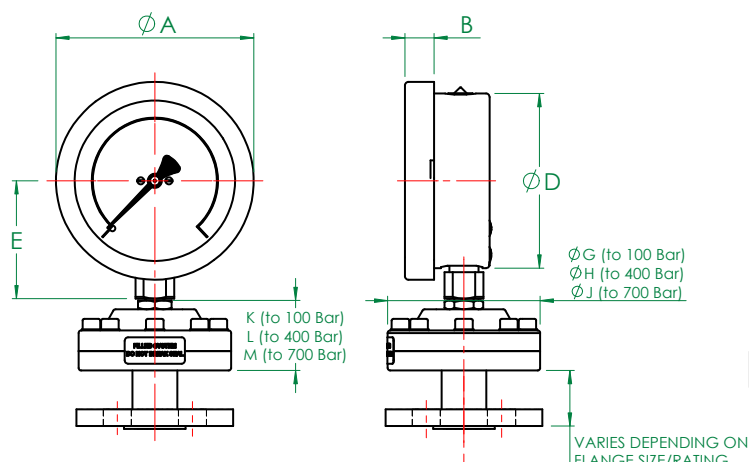
MODEL - 2033/F (below DN50/2") Flange Mounted - Rated as Flange to Maximum seal/chamber ratings
