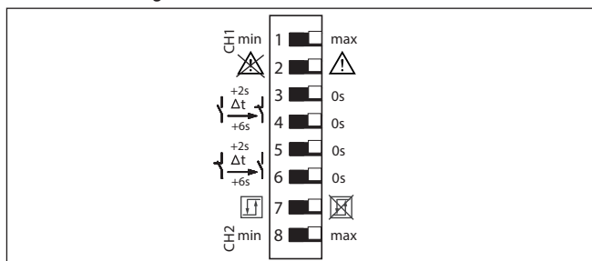
Fig. 3: DIL switch VEGATOR 122
