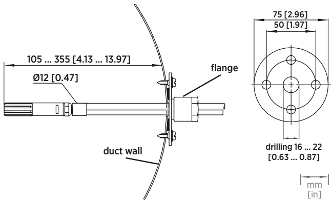
Left: Installation kit for duct mounting dimensions. Right: Installation flange dimensions. Aluminum or stainless steel.
