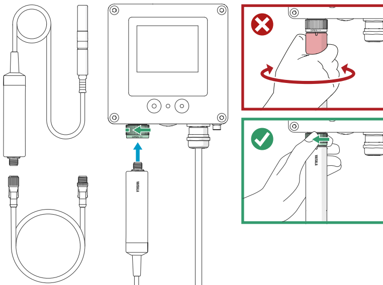
Figure 18 Connecting probe to Indigo300 transmitter
