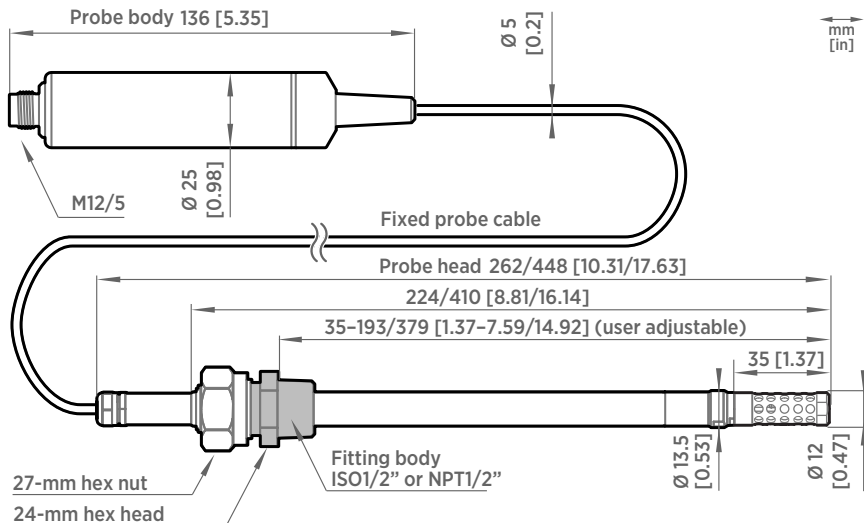
Figure 15 MMP8 dimensions
