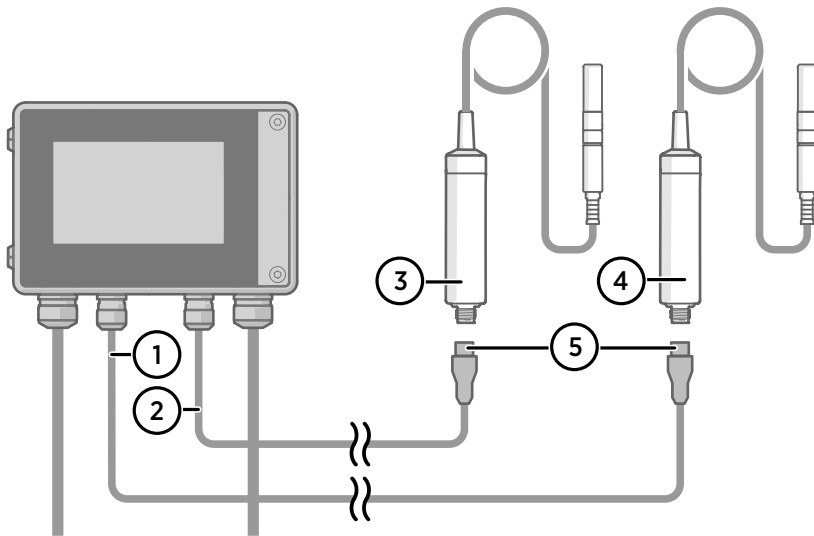
Figure 19 Connecting probes to Indigo500 transmitter
