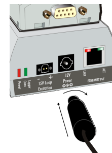
Figure 2 Connecting an external power supply
