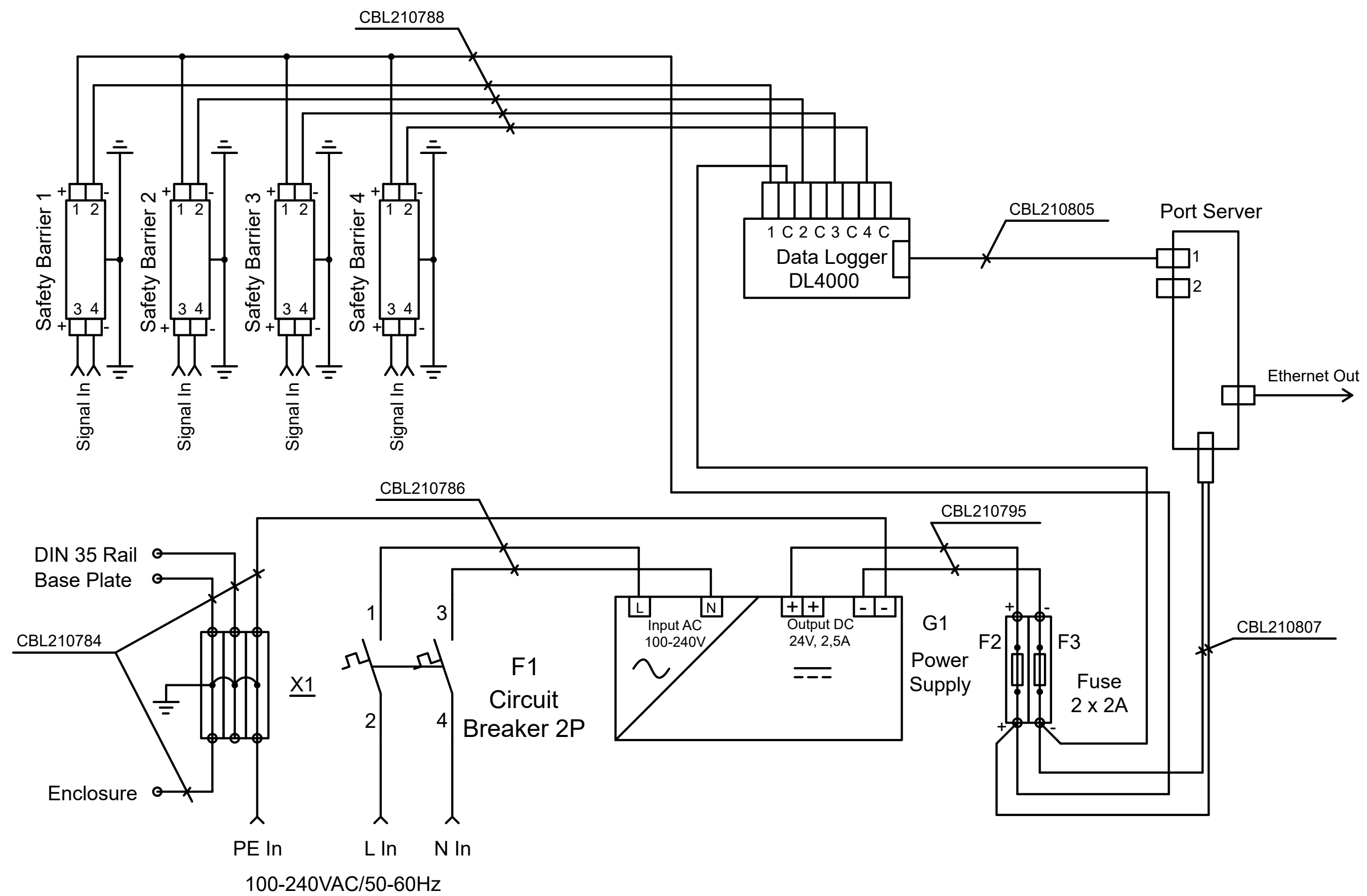
Wiring diagram for CAB100A safety barrier model with serial port server and 24 VDC power supply
