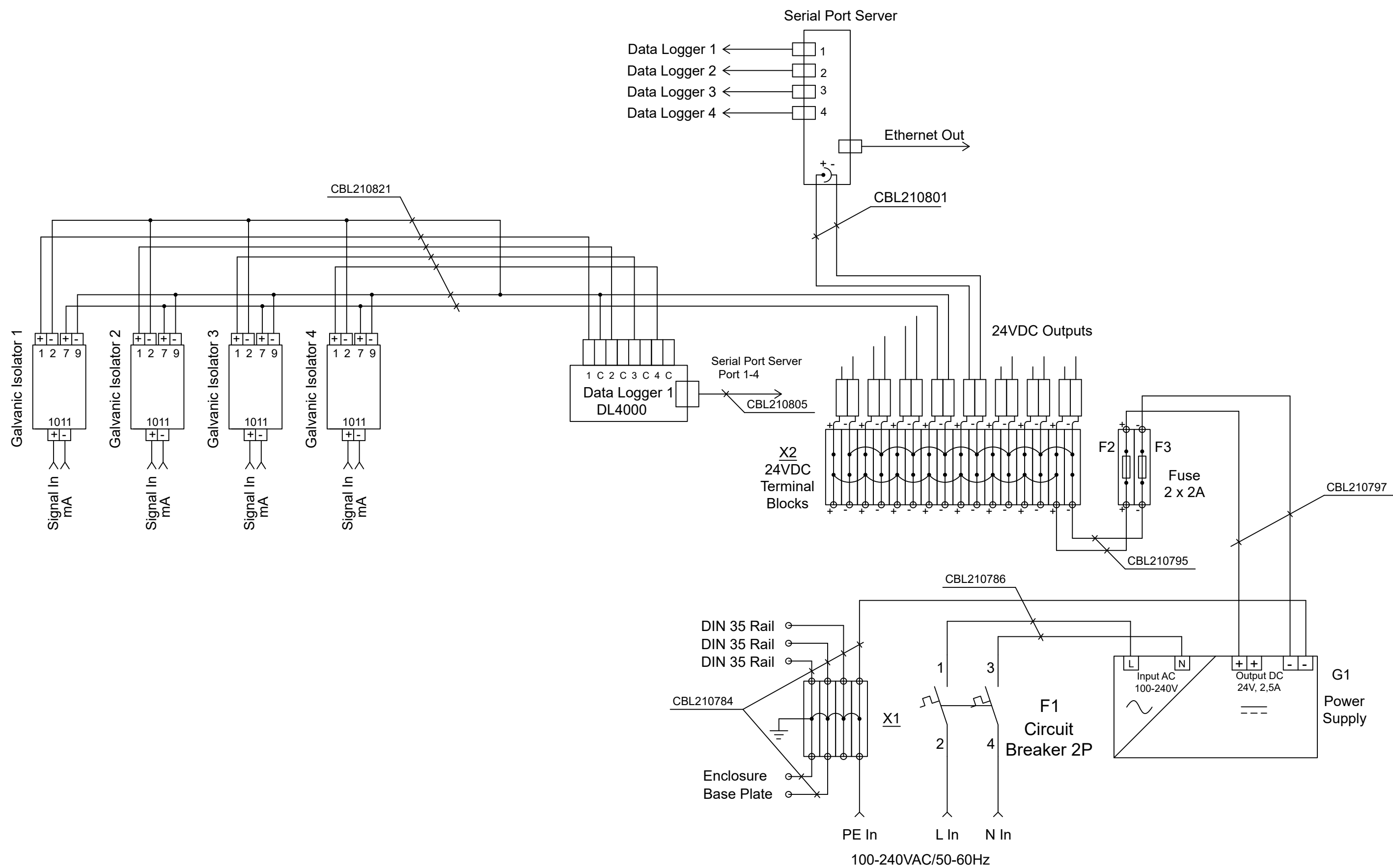
Wiring diagram for CAB100B galvanic isolator model
