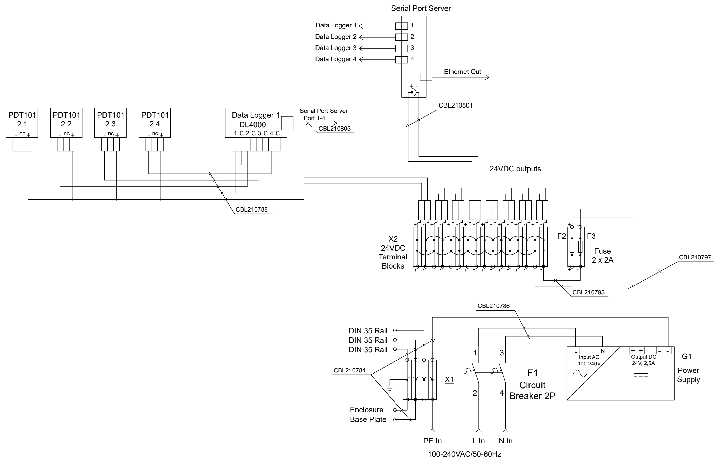
Wiring diagram for CAB100B PDT101 model
