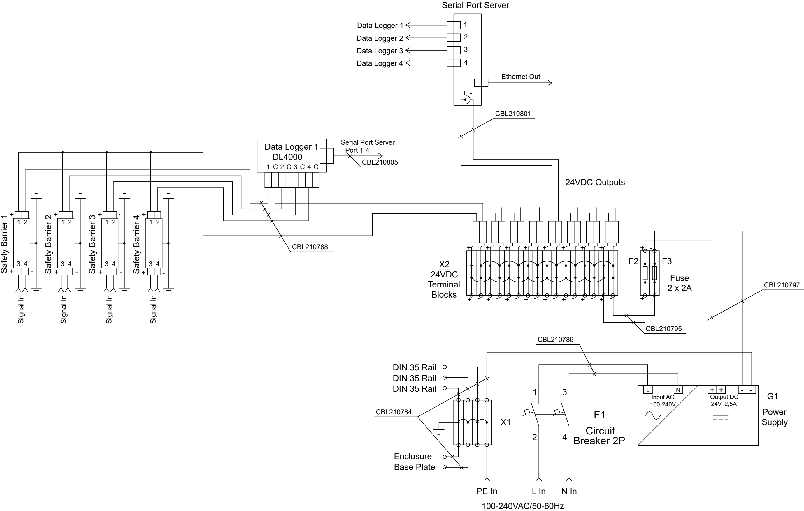
Wiring diagram for CAB100B safety barrier model
