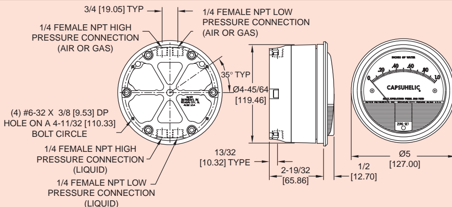
Dimensions, Series 4000 Capsuhelic® Pressure Gages.
