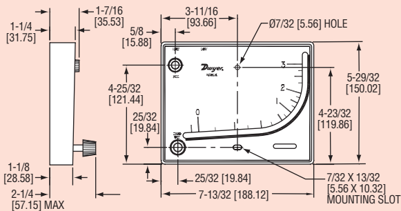
Fig. 13-2, Mark II Model No. 40-1 inclined manometer
