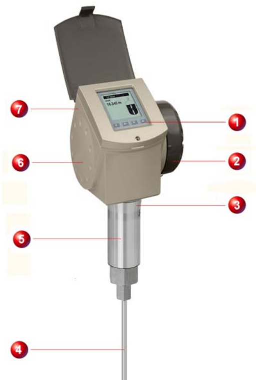
Figure 1 – SmartLine Guided Radar Level Meter
