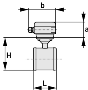
Front view VersaFlow (w/TWM9000F)
