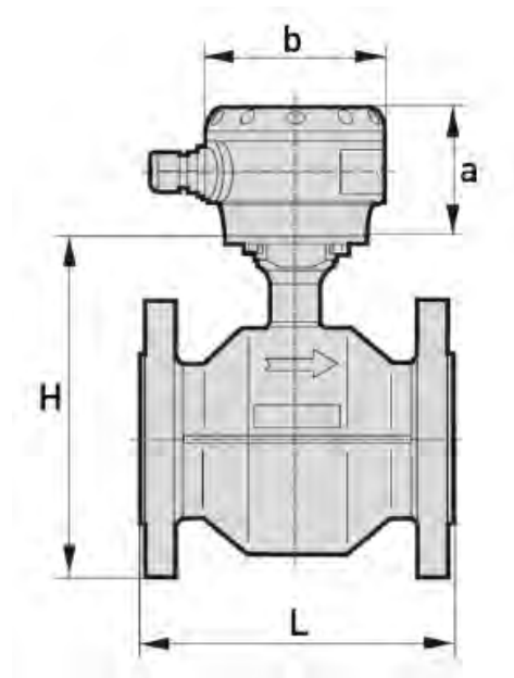
Frontview VersaFlow Mag 2000 F
