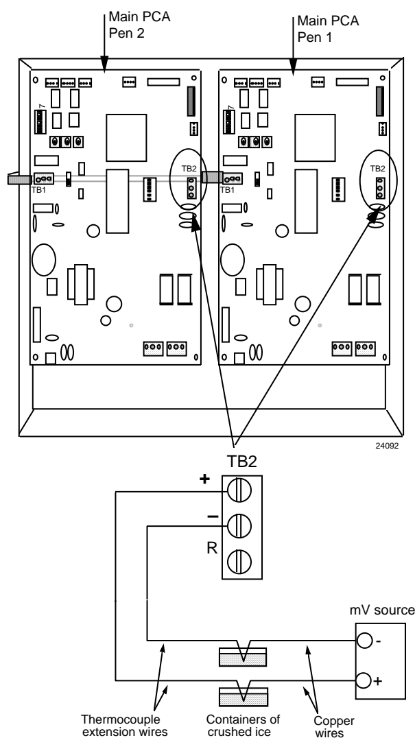
Figure 5-3 Calibration Set Up Diagram for Thermocouple Inputs Using an Ice Bath
