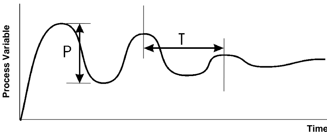
Figure 39. Manual Tuning
