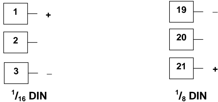
Figure 21. Option Slot 1 - Linear Voltage & mADC Module
