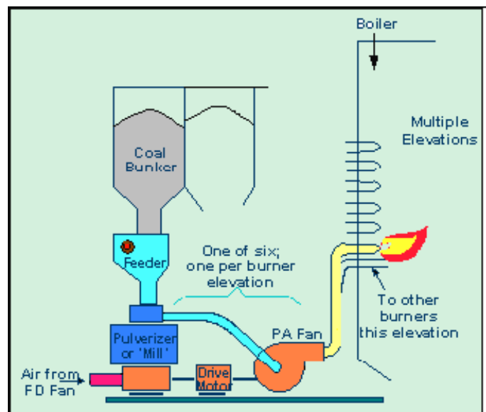
Figure 1. A typical mill/burner arrangement
