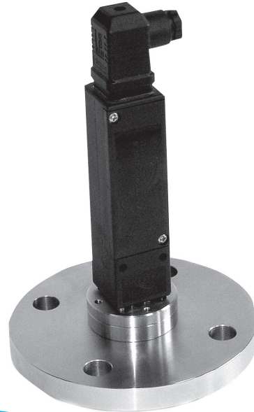
FLUSH DIAPHRAGM
